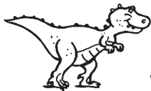
dinosaur
